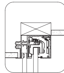
Option 7 Recessed sidelite, drywall x drop ceiling
