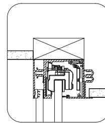
Option 6 Recessed cover, drywall x drop ceiling
