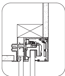
Option 4 Recessed sidelite, vertical drywall x drop ceiling
