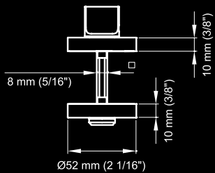
UEZ1332 - PB 83 cosmos black
