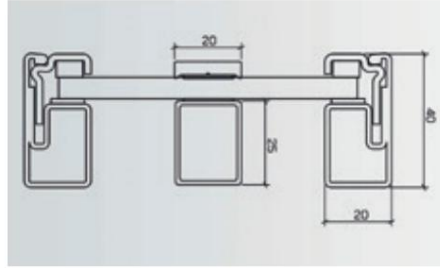
Construction rung, welded on one side
